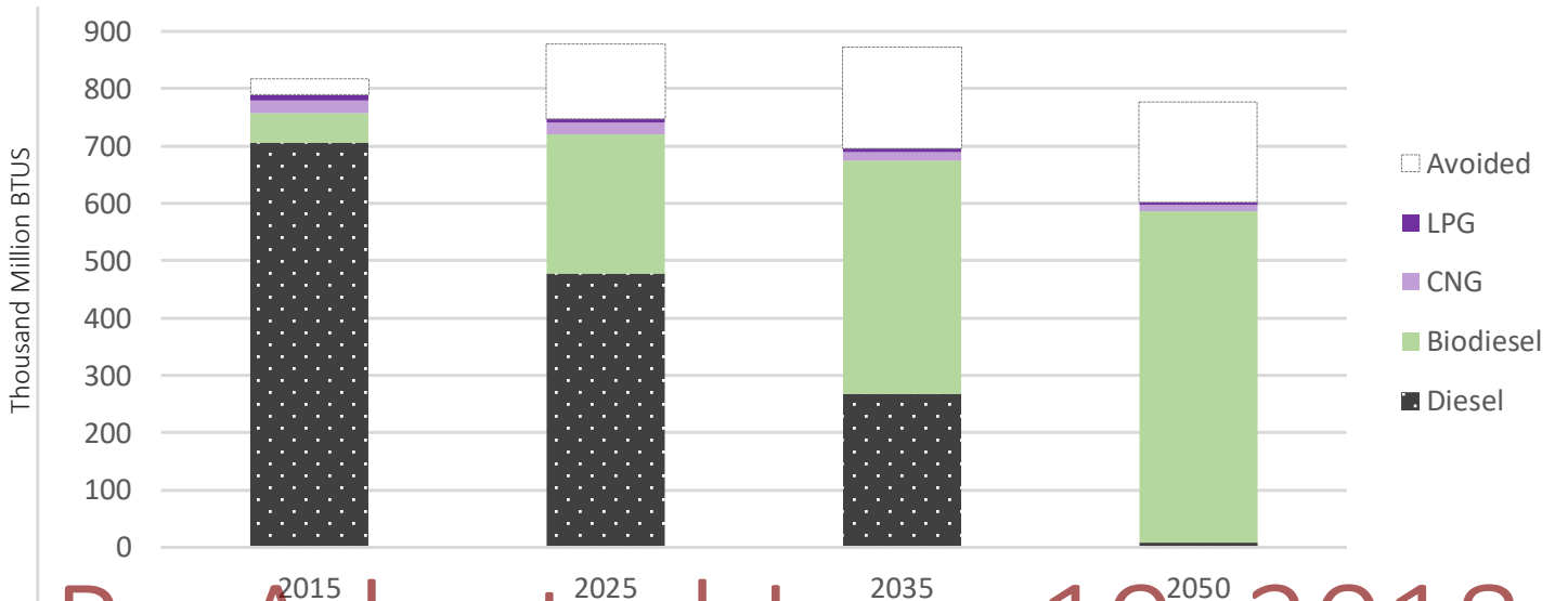
Rutland Region Heavy Duty Transportation Energy Consumption by Fuel 90 x 2050 VEIC Scenario Avoided vs Reference
